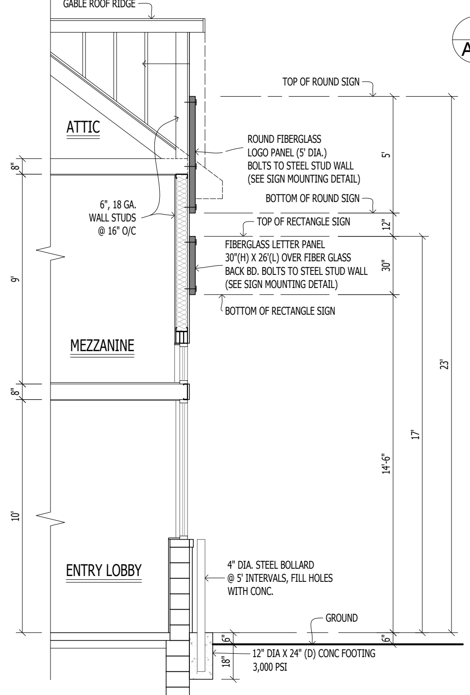
1 ELEVATION 1/8" = 1'-0"
