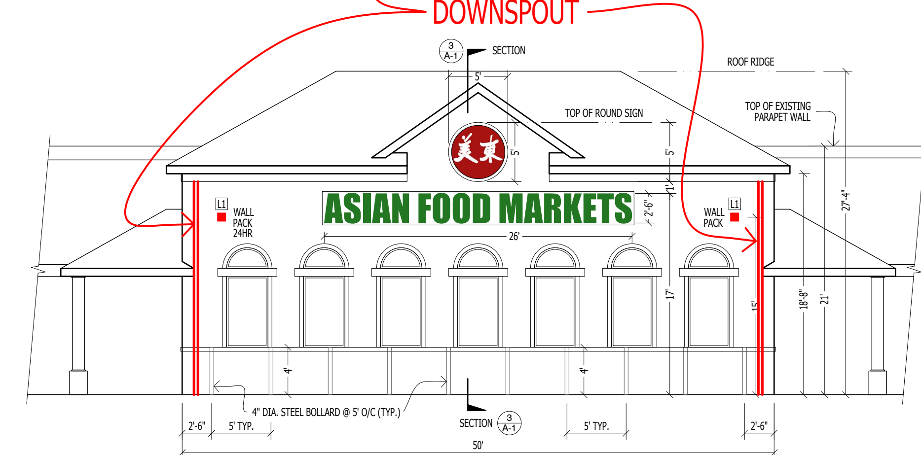
4 SIGN & BOLLARD ELEVATION 1/8" = 1'-0"
